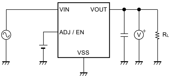
Figure 10 Test Circuit 7
