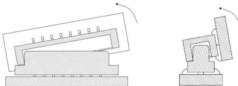
× 図-4 こじり抜去 (Not Good) Figure 4 Wthdrawal with twisting the connector at an angle
