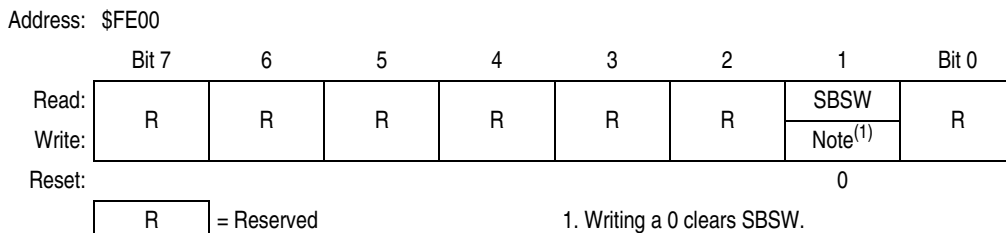
Figure 15-8. Break Status Register (BSR)
