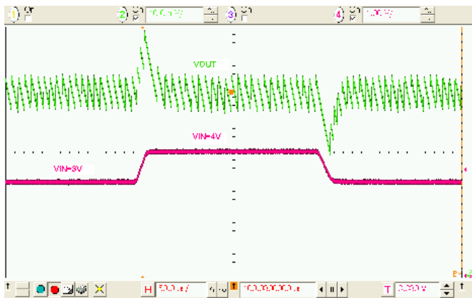
Figure 20. Line Transient, 50 Ω Load, t_R=t_F=10\ \mu\text{s}
