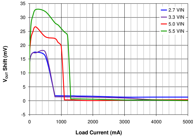
Figure 10. Regulation, 1.2 V OUT
