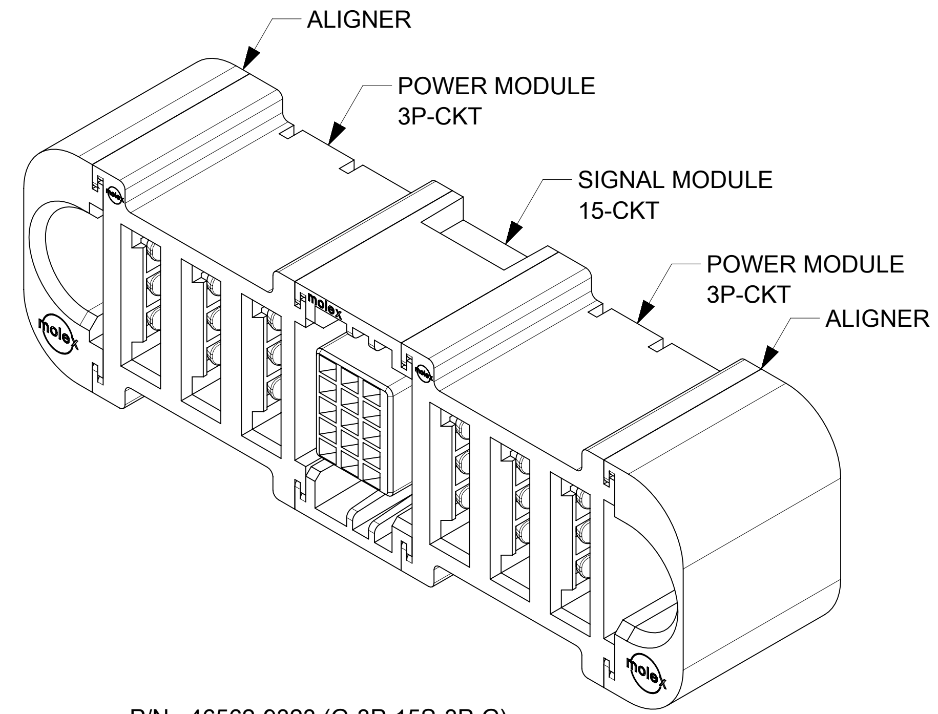
P/N : 46562-9323 (G-3P-15S-3P-G)
