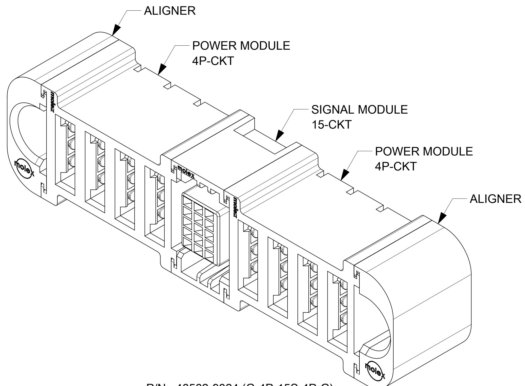
P/N : 46562-9324 (G-4P-15S-4P-G)
