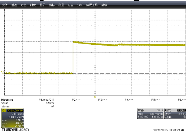
Fig:20 Vds = 5.92Vp-p at 3A at 90Vac
