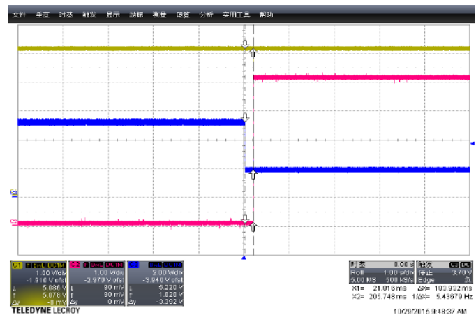
Fig:23 At 265Vac_Rising time = 184mS at 0A load
