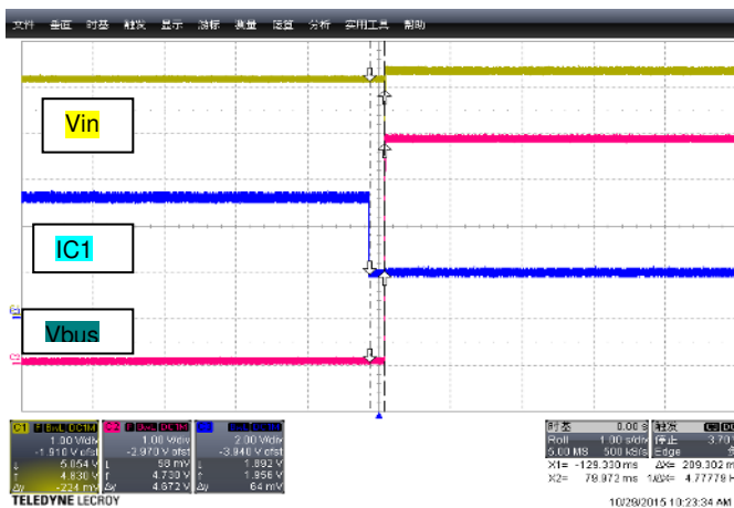
Fig:22 At 90Vac_Rising time =209mS at 3A load
