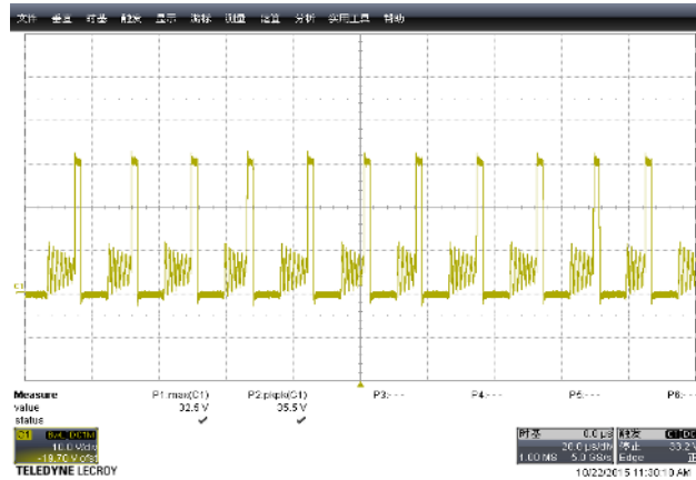
Fig:19 Vds = 35Vp-p at 3A at 265Vac
