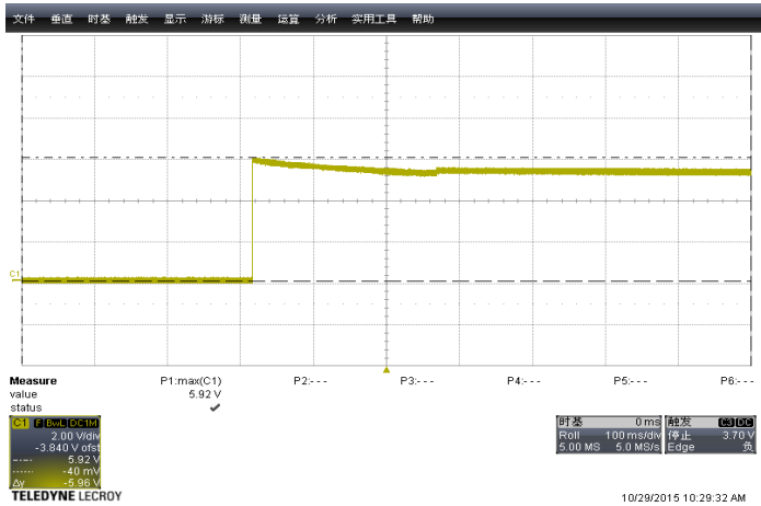
Fig:21 Vds = 5.91Vp-p at 3A at 265Vac
