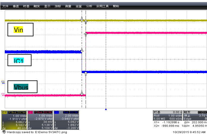
Fig:22 At 90Vac_Rising time =202mS at 0A load
