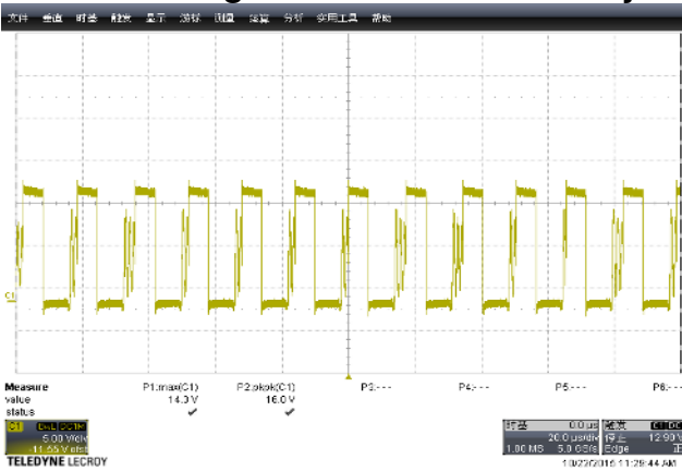
Fig:18 Vds = 18Vp-p at 3A at 90Vac
