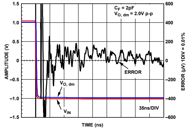
Figure 36. Settling Time (0.01%)
