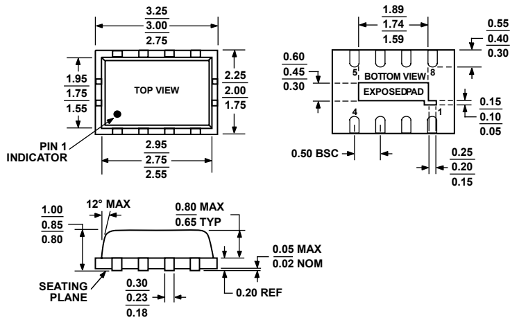
Figure 47. 8-Lead Lead Frame Chip Scale Package [LFCS_P_VD]
