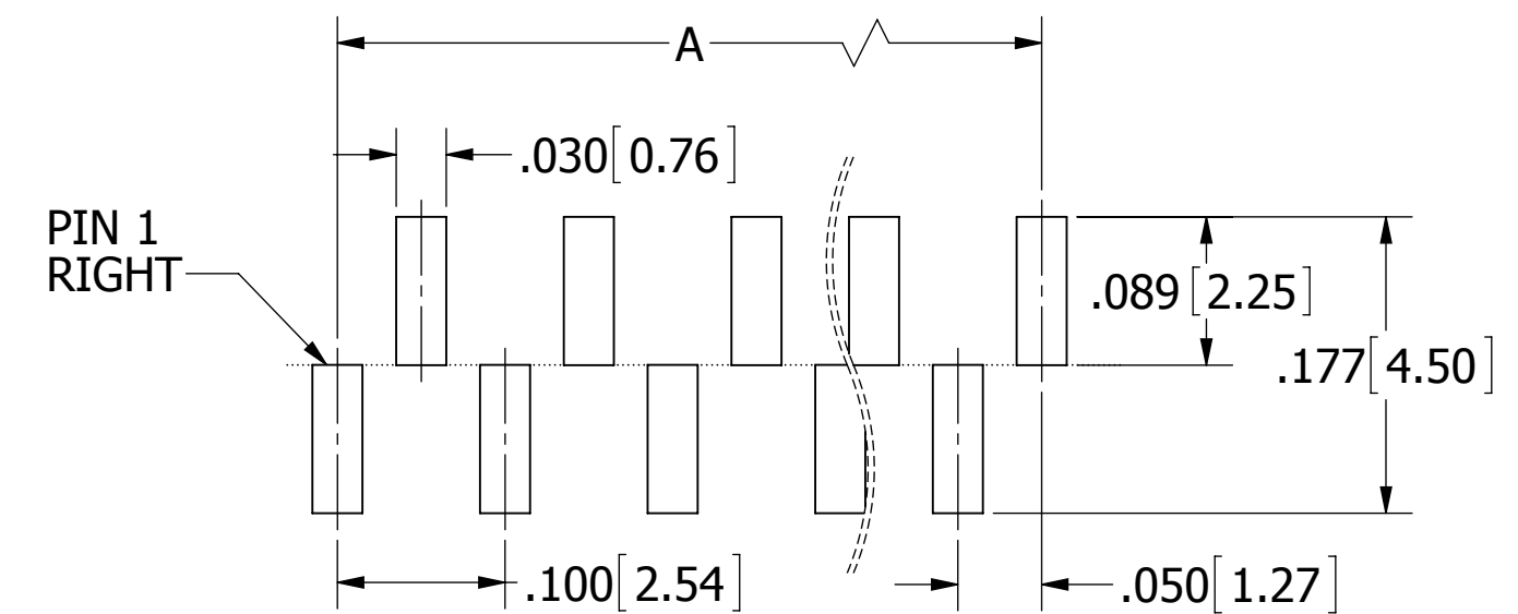
RECOMMENDED PCB LAYOUT GRP_1VWTD-RC
