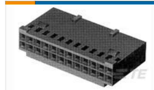
TE Part #87631-5 10 MODIV HSG COMP DR .100 POL REC
