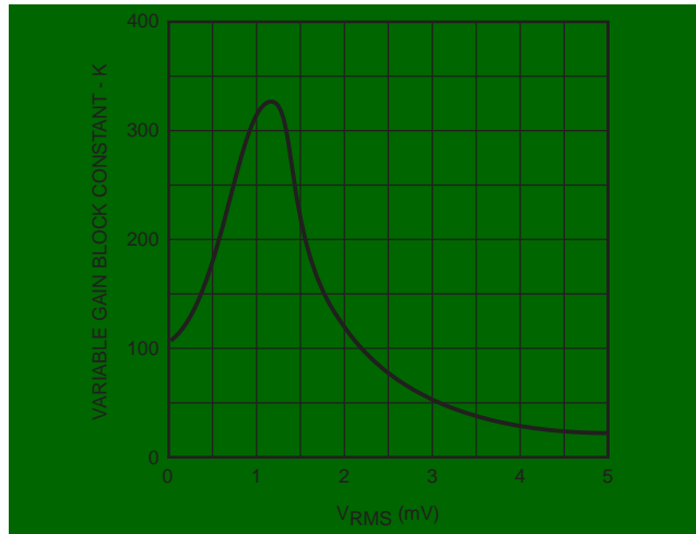
Gain Modulator Transfer Characteristic (K)
