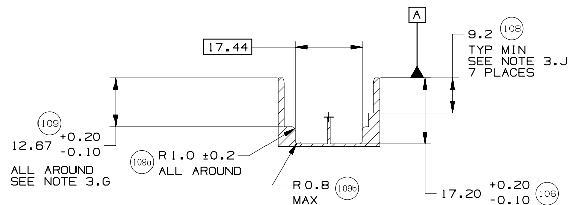
SECTION R-R
