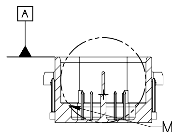
SECTION K - K
