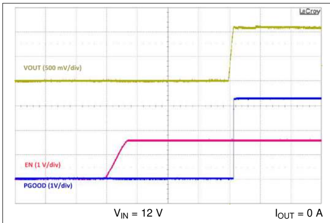
Figure 21. Enable Turn-on
