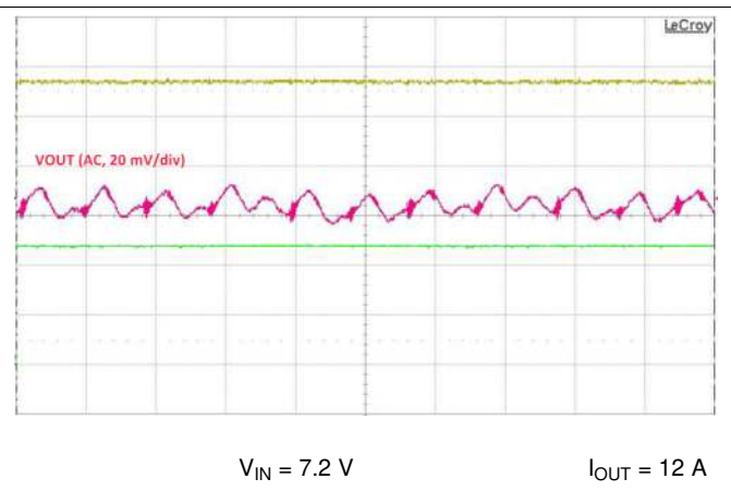
Figure 22. Output Ripple
