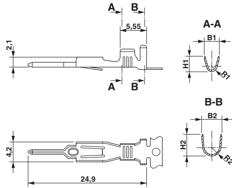
Dimensioned drawing
