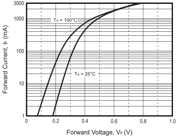
Fig.5 - Forward Characteristics
