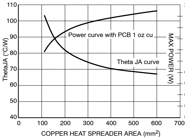
Figure 26. R_{\theta JA} vs. PCB Copper Area (DPAK)
