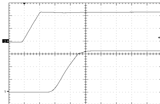
Figure 10. Startup Waveform via Input Voltage, time scale 2mS/div. Vin=Vin_nom, Iout=full load Cout=4700µF, Ch1=Vout (1V/div), Ch2=Vin (10V/div)
