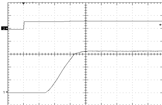
Figure 11. Startup Waveform via Enable Pin, time scale 2mS/div. Vin=Vin_nom, Iout=no load Cout=4700µF, Ch1=Vout (1V/div), Ch2=enable (10V/div)
