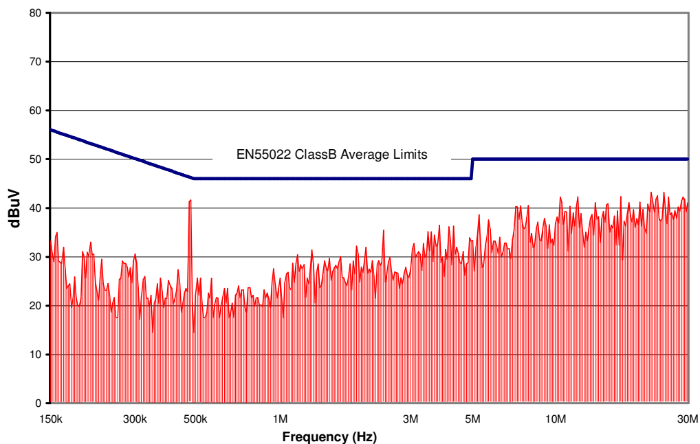
Figure 20. CP30_1775018 Conducted Emissions using above specified input filter. Vin = 24V, Full Resistive Load
