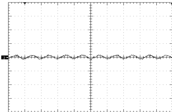
Figure 7. Input Reflected Ripple Current (10mA/div), time scale – 2µS/div. Vin=Vin_nom, full load (see Fig 15)
