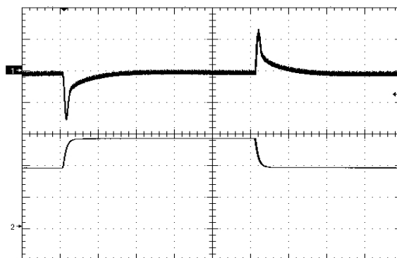
Figure 12. Load Transient Response (100mV/div), di/dt=0.1A/µS, 50%-75%-50% of full load, Cout=Fig16 time scale: 200µS/div. Ch1=Vout, Ch2=Iout (2A/div)
