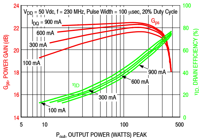
Figure 36. Power Gain and Drain Efficiency versus Output Power and Quiescent Current
