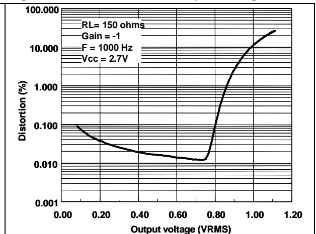
Figure 40. Distortion vs. output voltage
