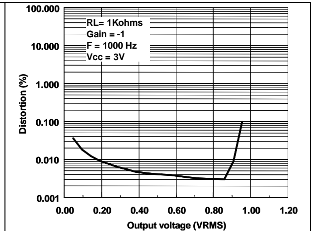
Figure 40. Distortion vs. output voltage
