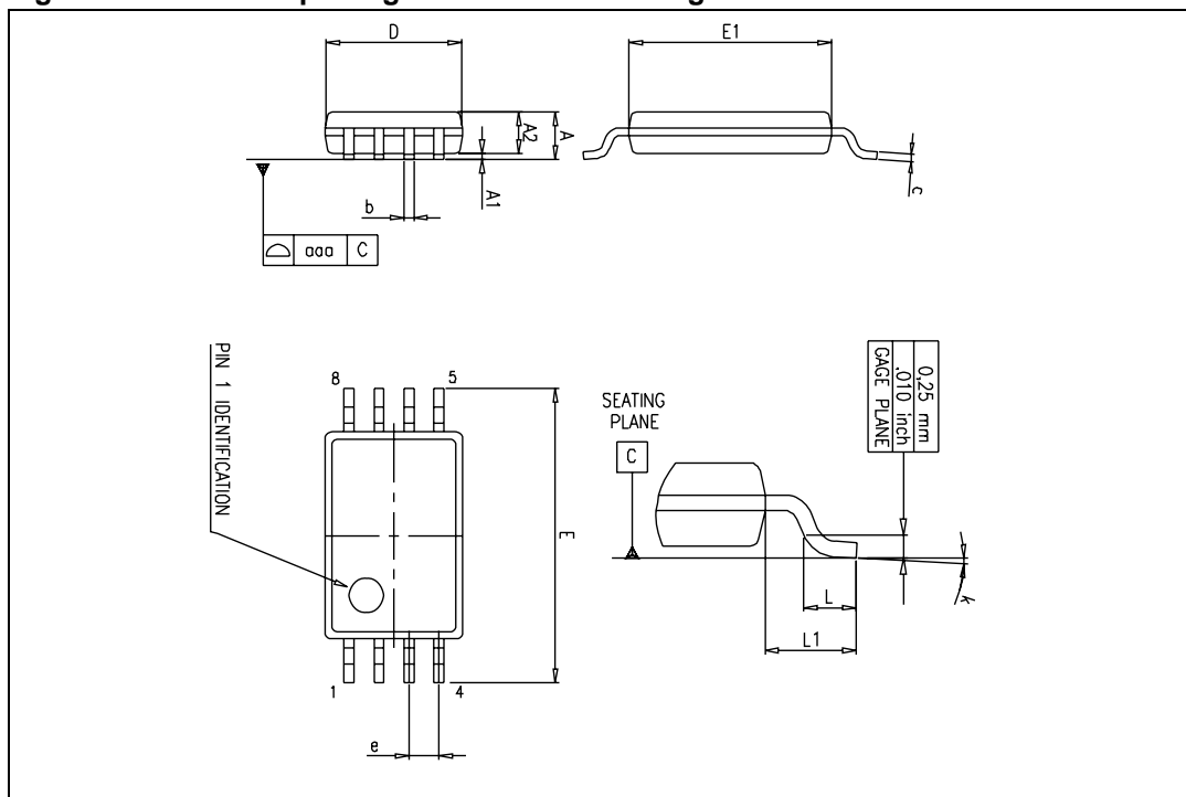
Figure 51. TSSOP8 package mechanical drawing
