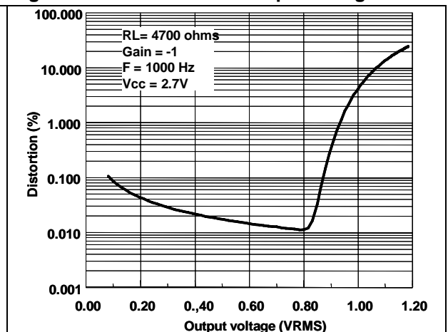
Figure 42. Distortion vs. output voltage
