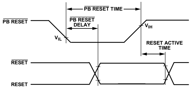
Figure 7. \overline{\text{PB RESET}}
