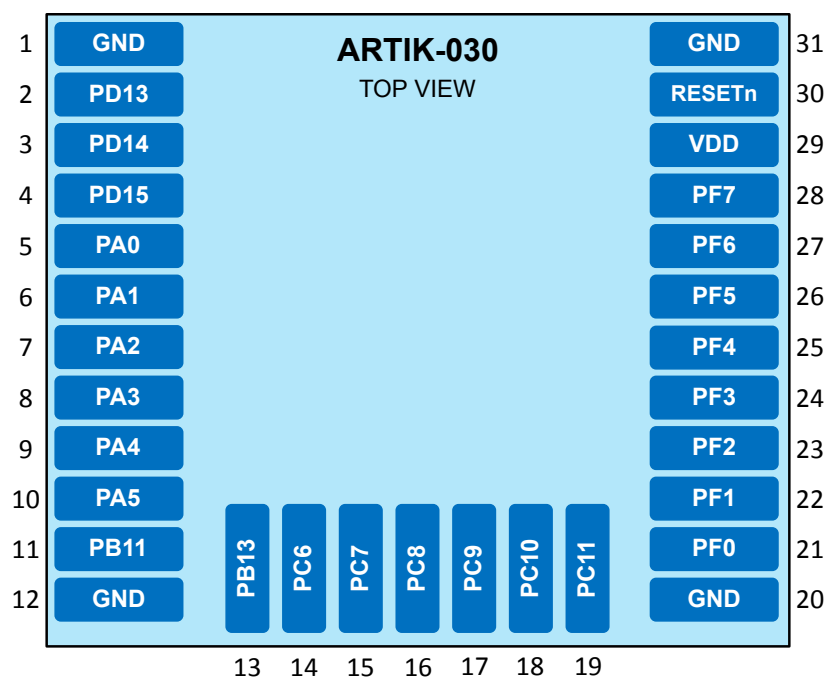
Figure 8.1. ARTIK 030 Pinout
