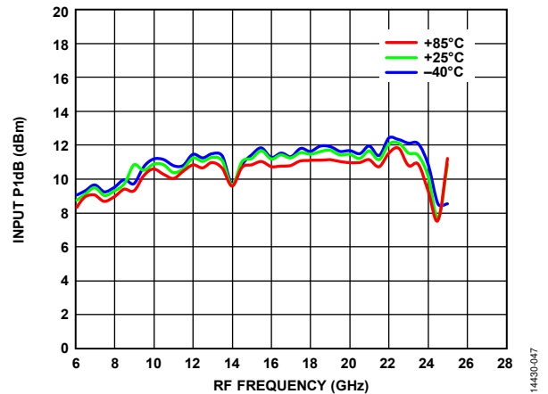
Figure 49. Input P1dB vs. RF Frequency at Various Temperatures, IF = 3000 MHz, LO Drive = 13 dBm, Lower Sideband
