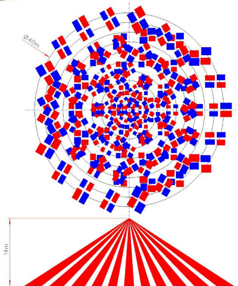
Diagram shows theoretical zone plot for detector mounted 14m above floor. Mounting height can be reduced as required. When used with a quad pyro the lens will project 516 individual detection zones within a 40m diameter circular area.
