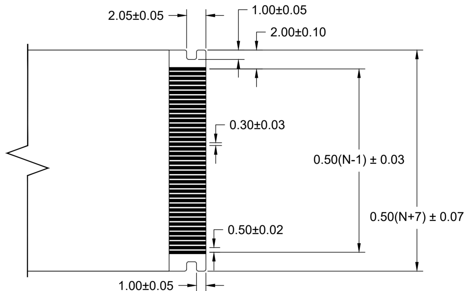
END TAIL DETAIL SCALE 4:1
