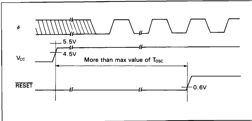
Figure 7. CPU Timing
