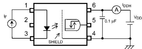
Fig. 13.1.4 I_{DDH} Test Circuit
