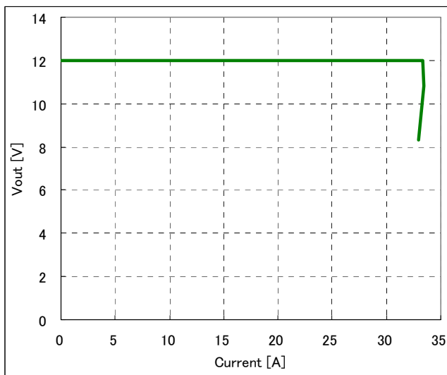
Fig-11: Output voltage vs. load current showing current limit point and converter shutdown point. ( V_{in} = 48\text{V} )
