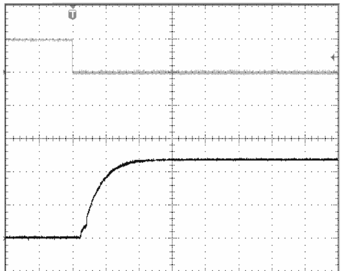
Fig-5: Turn-on transient at full rated load current (resistive) plus 10,000µF at Vin=48V, triggered via ON/OFF pin. Top trace: ON/OFF signal (5V/div). Bottom trace: output voltage (5V/div). Time scale: 10ms/div
