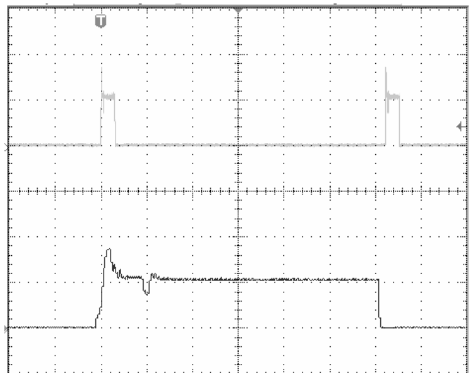
Fig-12: Load current (top trace, 20A/div, 40ms/div) into a 10\text{m}\Omega short circuit during restart, at V_{in} = 48\text{V} . Bottom trace (20A/div, 2ms/div) is an expansion of the top trace.
