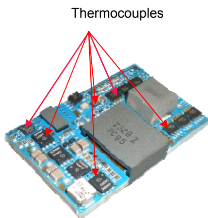
Fig. G: Location of thermocouples for thermal testing
