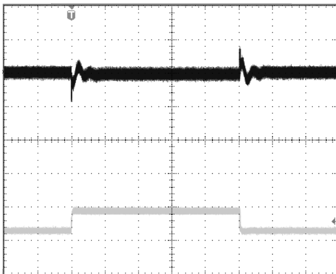
Fig-6: Output voltage response to load current step-change (15A-22.5A-15A) at Vin=48V. Top trace: Output voltage (200mV/div). Bottom trace: load current (10A/div). Current slew rate: 5A/µs. Co=470µF Low Z EL-con + 1 µ F ceramic. Time scale: 200µs/div
