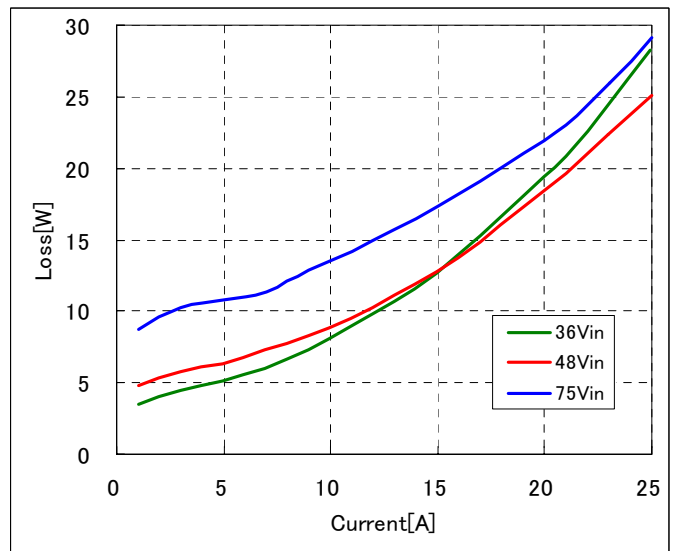
Fig-3: Power dissipation vs. load current and input voltage for converter mounted horizontally with airflow from pin 3 to pin 1 at a rate of 400LFM (2.0m/s) and Ta=25°C.
