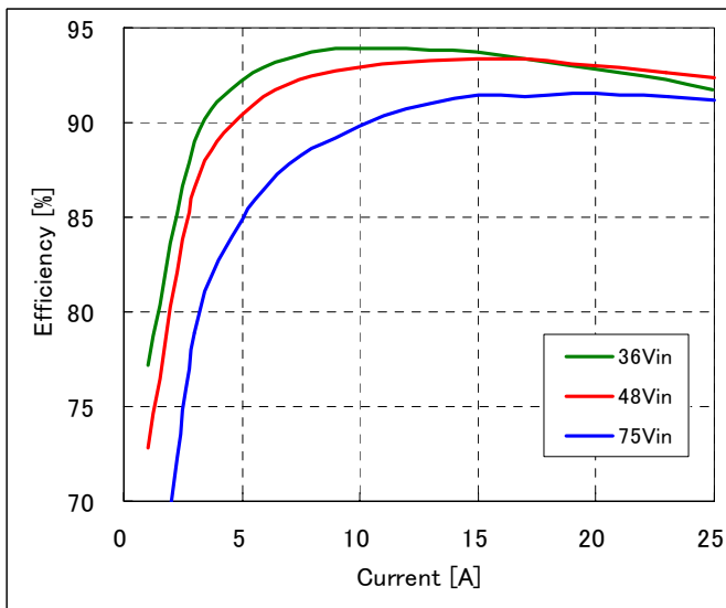
Fig-2: Efficiency vs. load current and input voltage for converter mounted horizontally with airflow from pin 3 to pin 1 at a rate of 400LFM (2.0m/s) and Ta=25°C.
