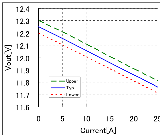
Graph-1 : Characteristic of output current vs output voltage in the parallel option
