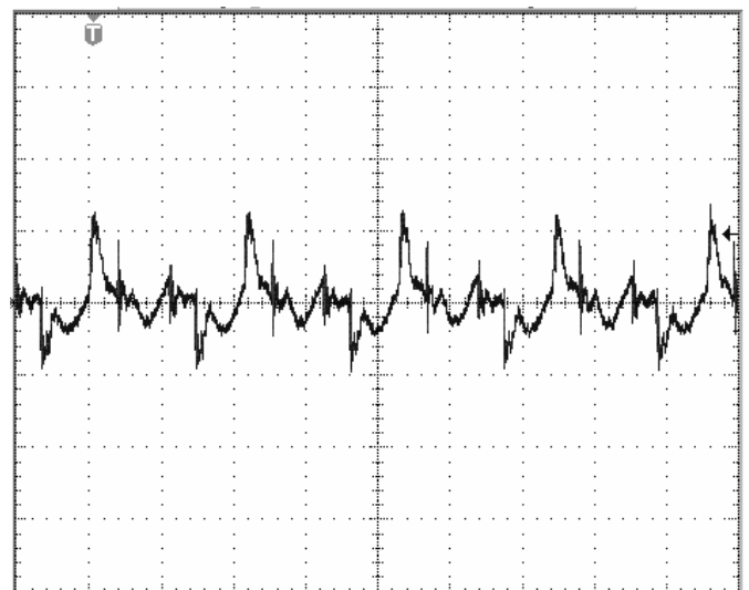
Fig-7: Output voltage ripple (50mV/div) at full rated load current into a resistive load with Co=10µF tantalum + 1 µ F ceramic and Vin=48V. Time scale: 1µs/div
