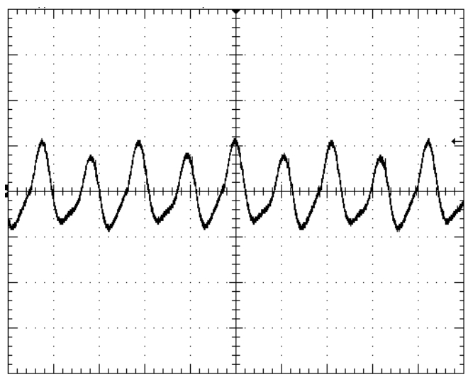
Fig-10: Input reflected ripple current, I_c (500mA/div), measured through 10\mu\text{H} at the source at full rated load current and V_{in}=48\text{V} . Time scale: 1\mu\text{s}/\text{div} .
