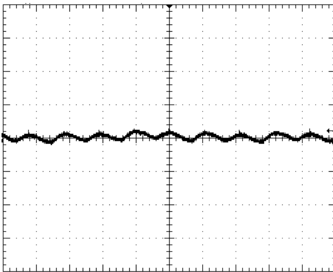
Fig-9: Input reflected ripple current, I_s (10mA/div), measured through 10\mu\text{H} at the source at full rated load current and V_{in}=48\text{V} . Time scale: 1\mu\text{s}/\text{div} .
