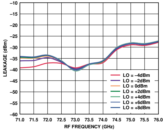
Figure 34. 6x LO Leakage at RFOUT vs. RF Frequency at Various LO Powers, IFIN = 5 dBm, IF = 500 MHz, LSB
