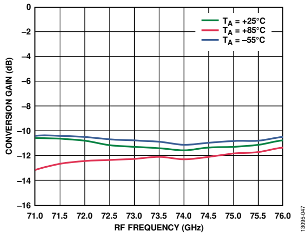
Figure 46. Conversion Gain vs. RF Frequency at Various Temperatures, I_{FIN} = -8 dBm, LO = 2 dBm, IF = 500 MHz, USB
