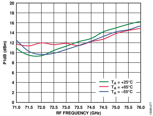
Figure 76. Input P1dB vs. RF Frequency at Various Temperatures, LO = 2 \text{ dBm} , IF = 2000 \text{ MHz} , USB
