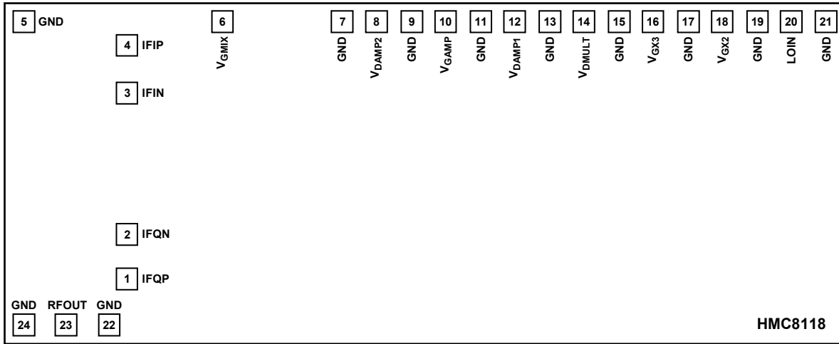
Figure 2. Pad Configuration
