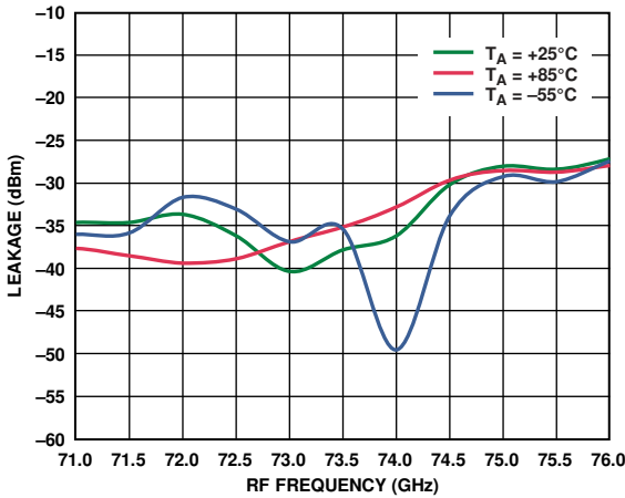
Figure 31. 6x LO Leakage at RFOUT vs. RF Frequency at Various Temperatures, IFIN = 5 dBm, LO = 2 dBm, IF = 500 MHz, LSB
