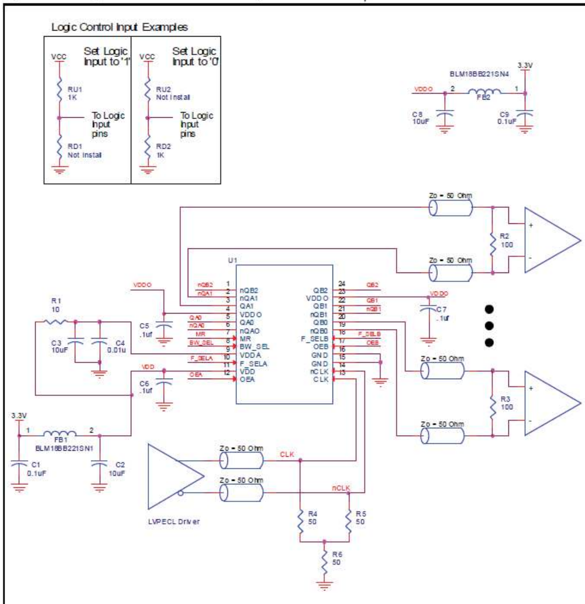
FIGURE 5. 874005 SCHEMATIC EXAMPLE
