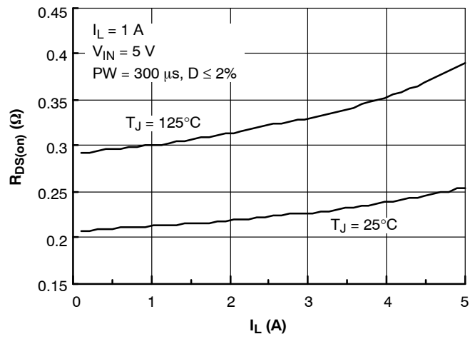
Figure 6. R_{\text{DS(on)}} Versus I_L at V_{\text{IN}} = 5.0 \text{ V}
