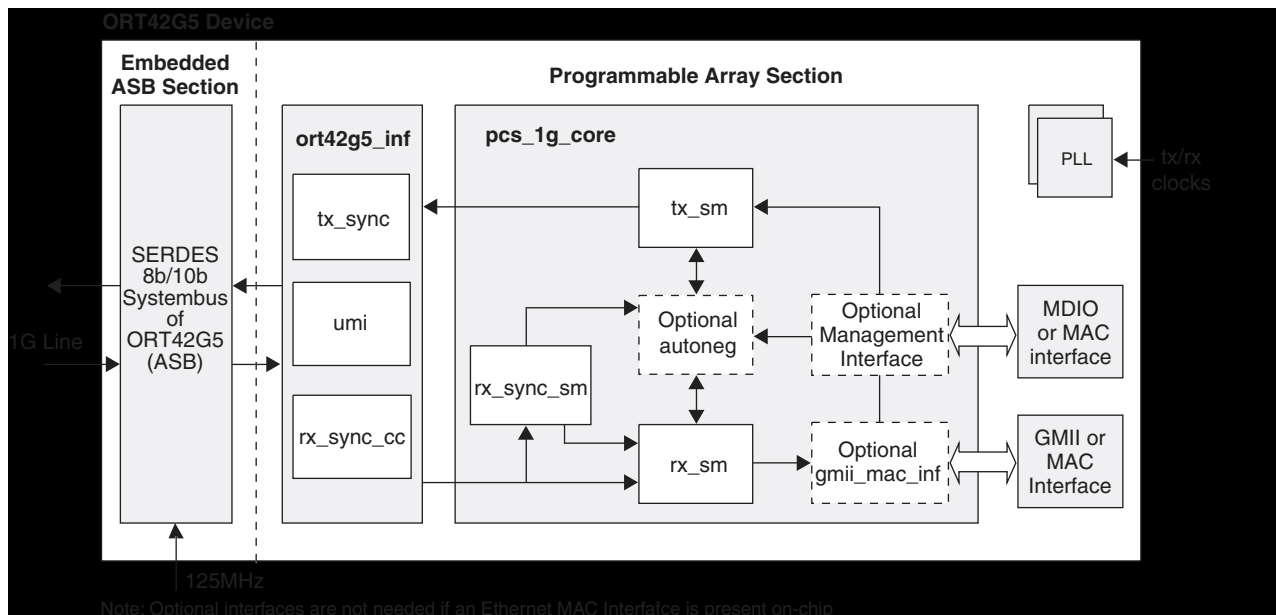
Figure 1. 1GbE PCS Solution
