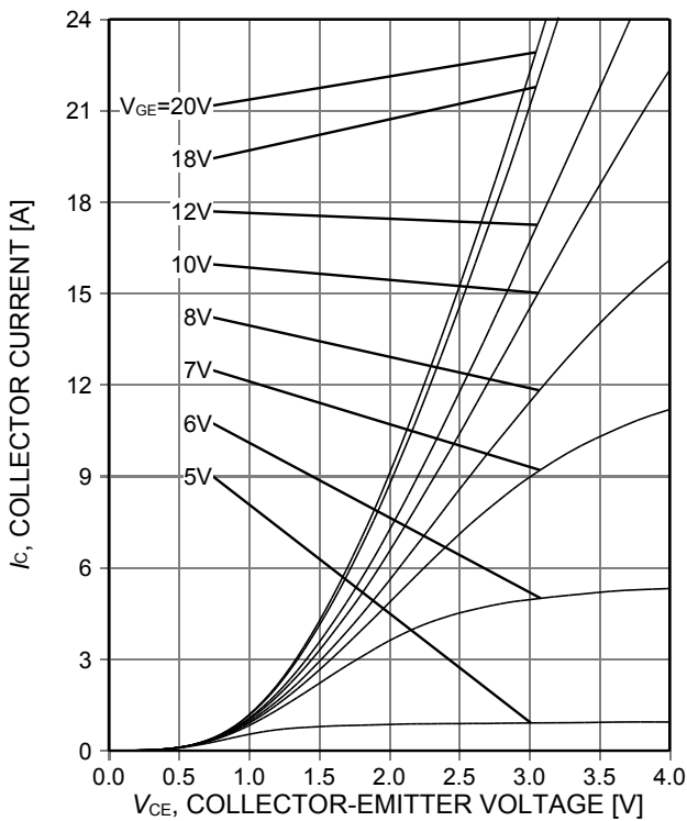
Figure 5. Typical output characteristic ( T_{j}=150^{\circ}\text{C} )
