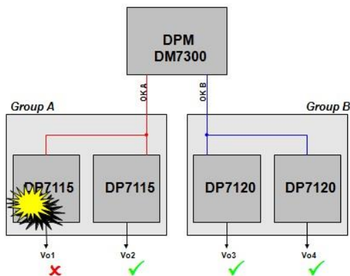
Figure 35. No Group Fault Propagation
