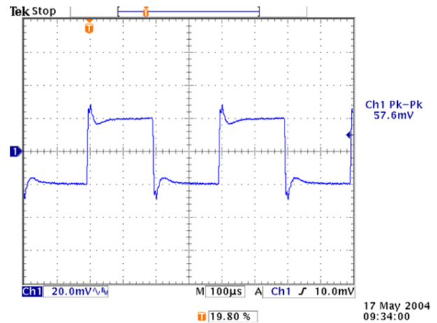
Figure 15. Transient Response with Optimal Voltage Positioning
