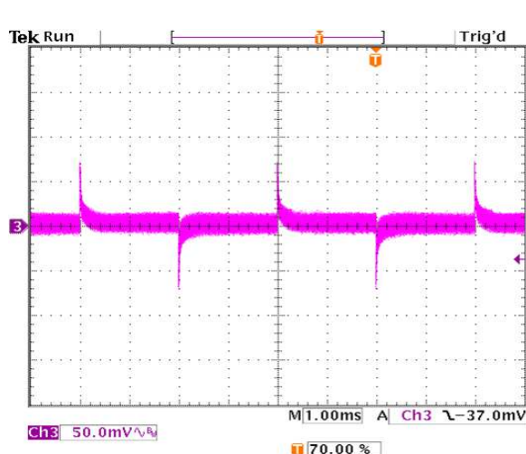
Figure 47. Transient Response with Regulation set to 0.0 mV/A Figure 48. Transient Response with Regulation set to 1.48 mV/A
