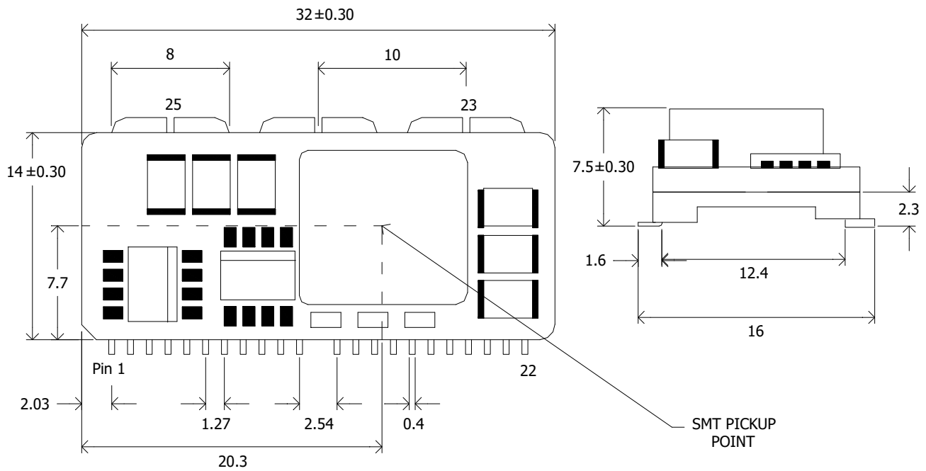
Figure 52. Mechanical Drawing
