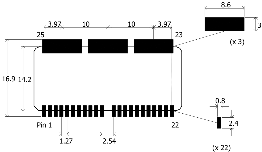
Figure 53. Recommended Pad Sizes
