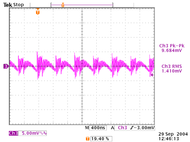
Figure 45. Output Voltage Noise, Full Load, 180° Interleave
