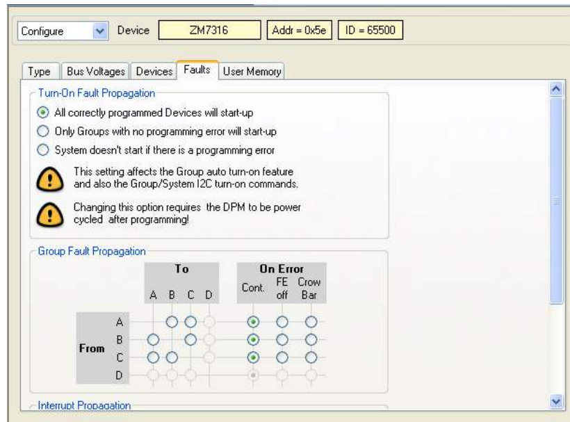
Figure 33. DPM Configure Faults Window
