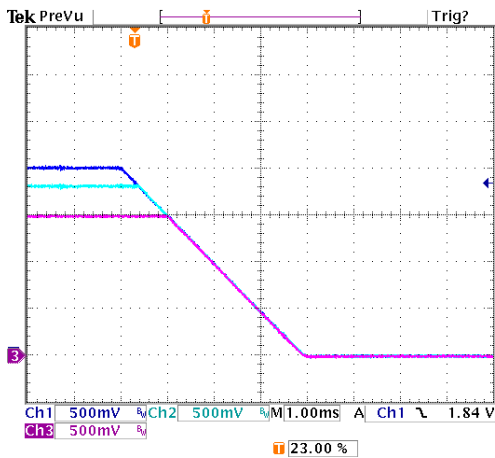
Figure 26. Tracking Turn-Off. Falling Slew Rate is programmed at 0.5V/ms.
