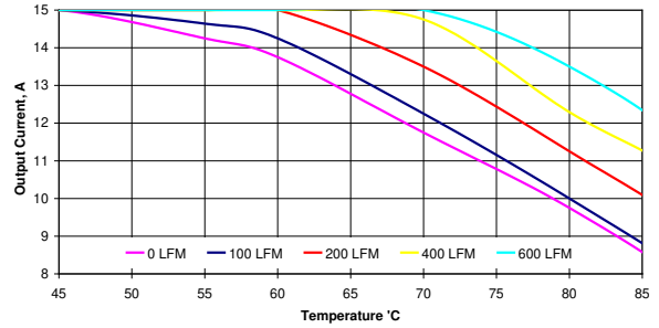
Figure 10. Thermal Derating Curves. Vin=13.2V, Vout=5.0V, Fsw=1MHz
