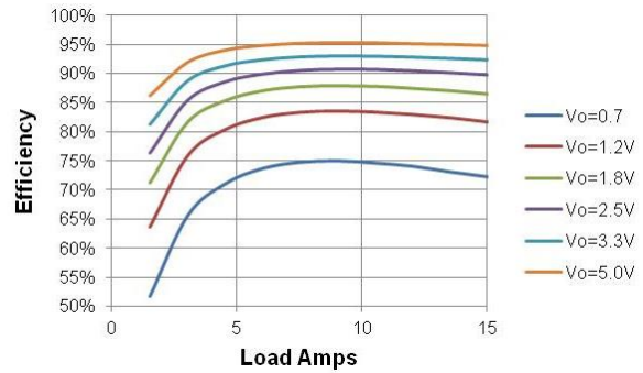
Figure 4. Efficiency vs. Load. V_{in}=8V , F_{sw}=1MHz
