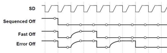
Figure 39. OK Severity Encoding Waveforms
