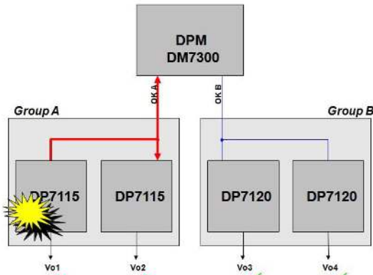
Figure 37. Intra Group Fault Propagation
