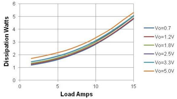
Figure 8. Dissipation vs Load, Vin=12V, Fsw=1MHz
