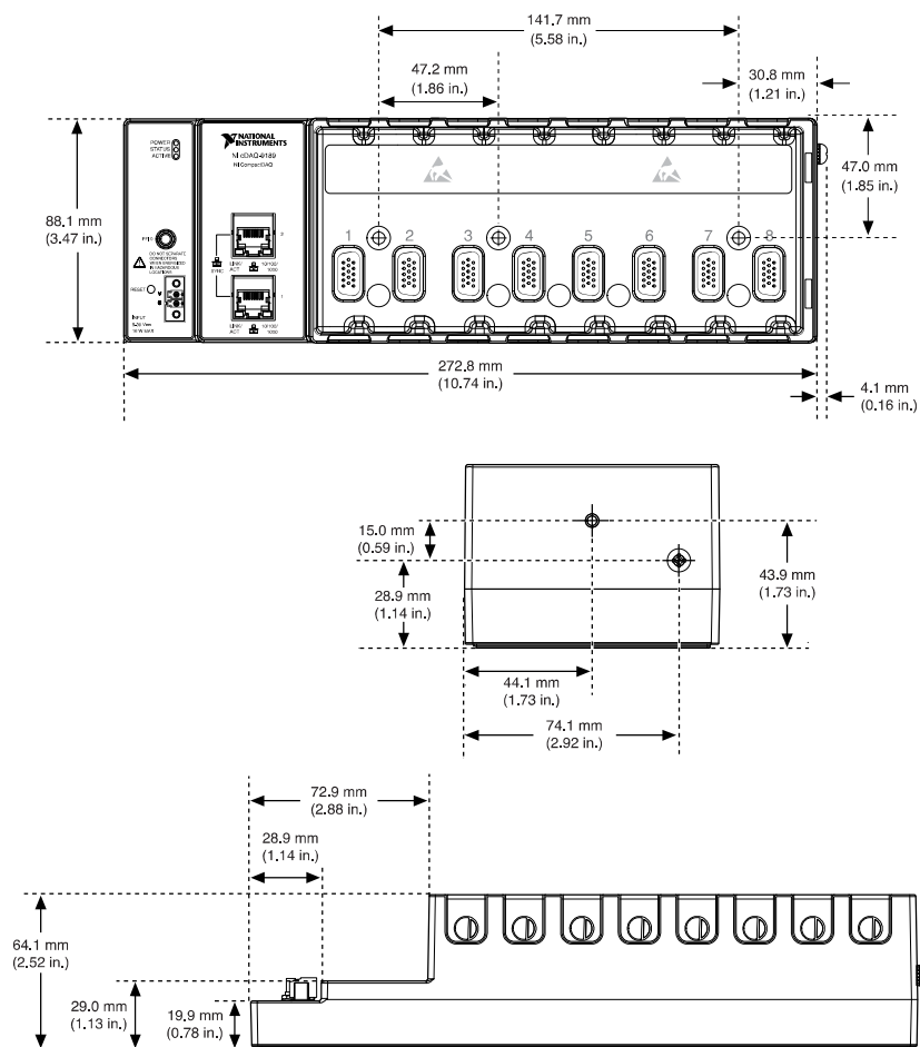
Figure 1. cDAQ-9189 Dimensions
