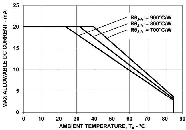
Figure 6: Derating Curve
