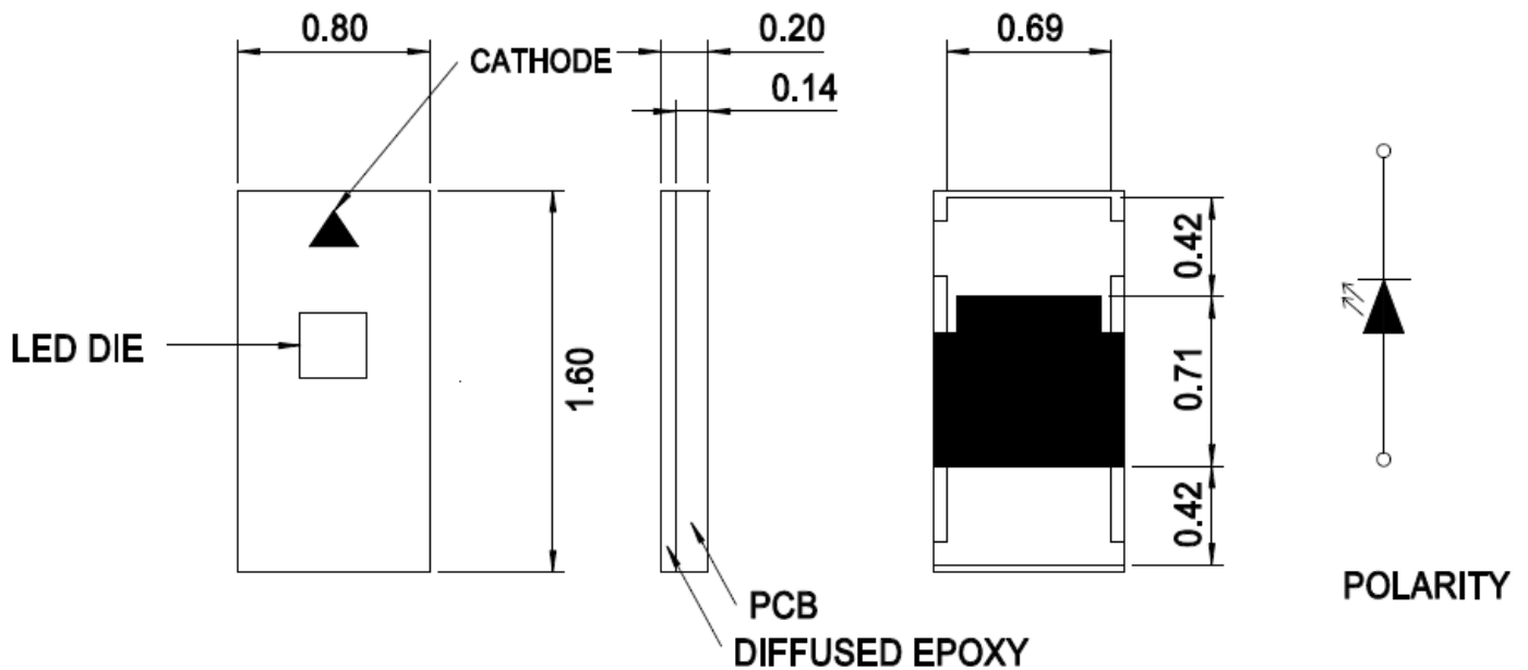
Figure 1: Package Dimensions
