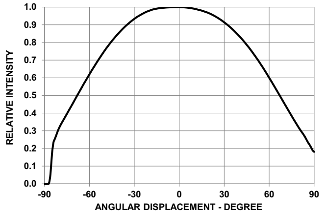
Figure 5: Radiation Pattern
