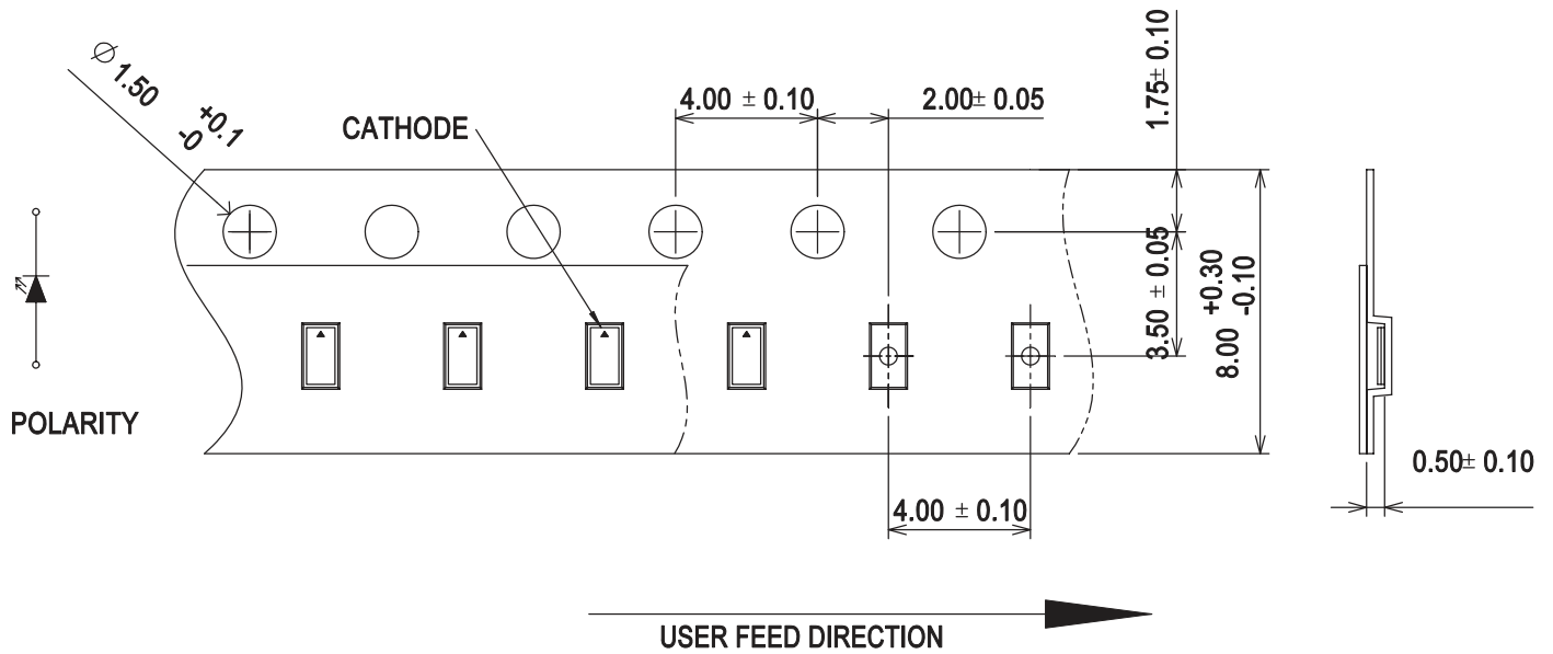
Figure 8: Carrier Tape Dimensions
