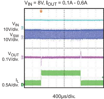
Load Transient
