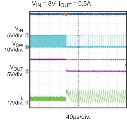
Short Output
