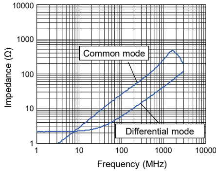
● EXC24CG240U
