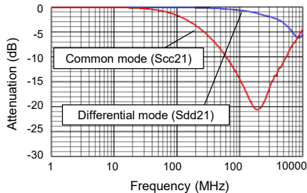
● EXC24CG240U
