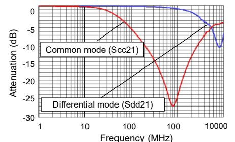
● EXC24CG900U
