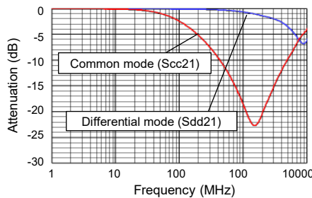
● EXC24CG360U
