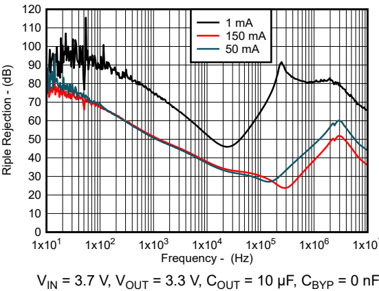
V_{IN} = 3.7\text{ V} , V_{OUT} = 3.3\text{ V} , C_{OUT} = 10\text{ }\mu\text{F} , C_{BYP} = 0\text{ nF} Figure 6-21. Ripple Rejection vs Frequency for New Chip
