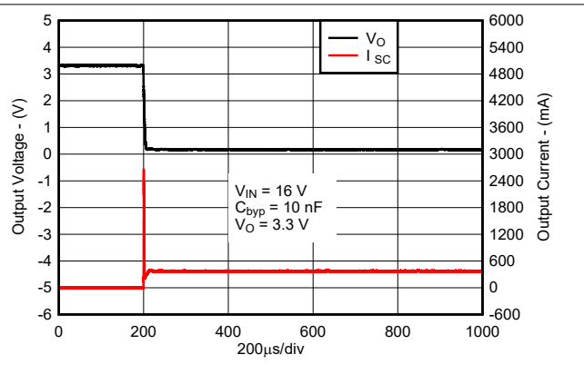
Figure 6-12. Short-Circuit Current vs Time for New Chip
