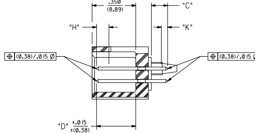
SECTION Z-Z
