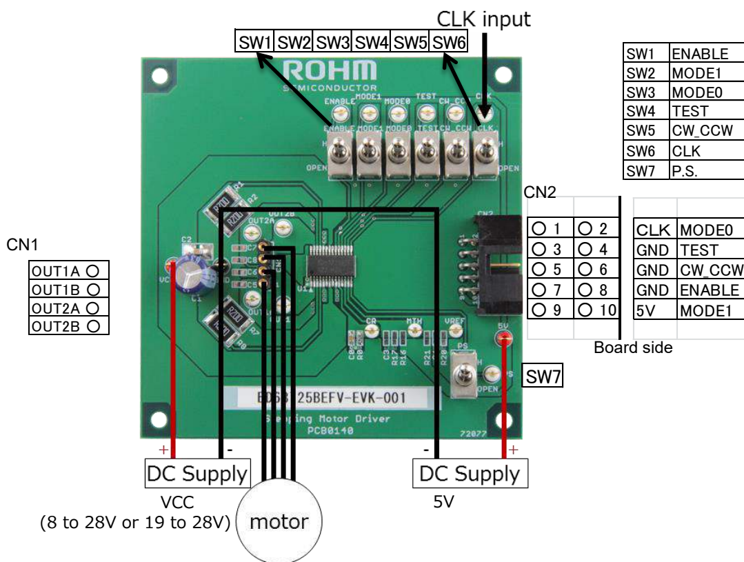
Figure 4. Motor Connection
