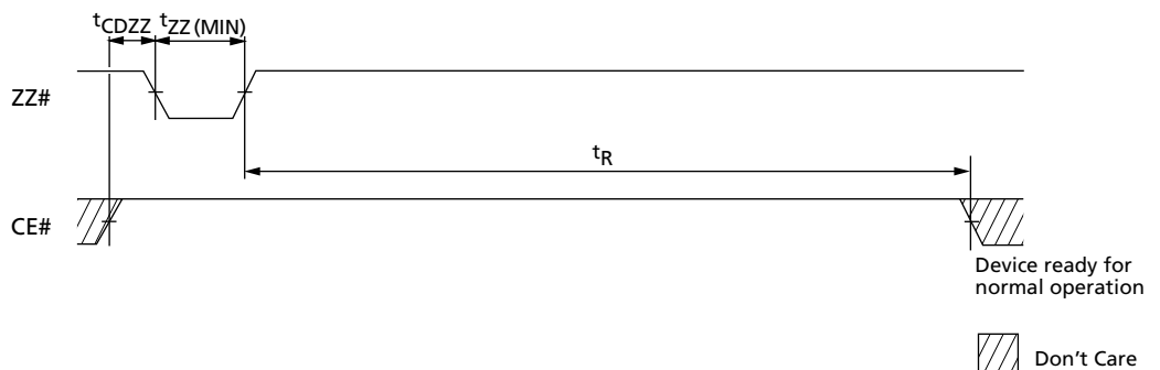
Figure 18: Deep Power-Down n Entry and Exit
