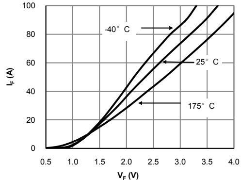
Fig 4: Diode Characteristic
