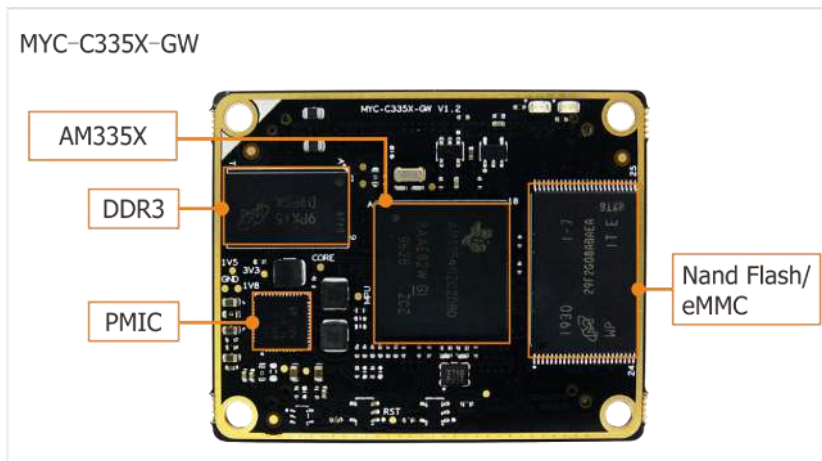
MYC-C335X-GW CPU Module
