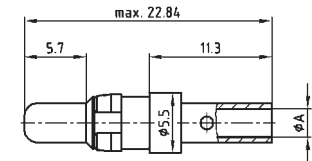
Plug contact
