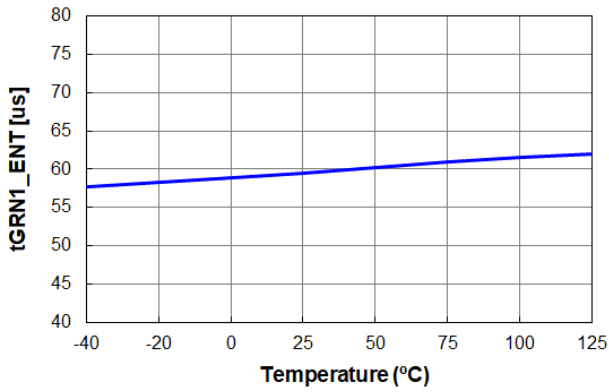
Figure 41. t_{\text{GRN1-ENT}} vs. Temperature
