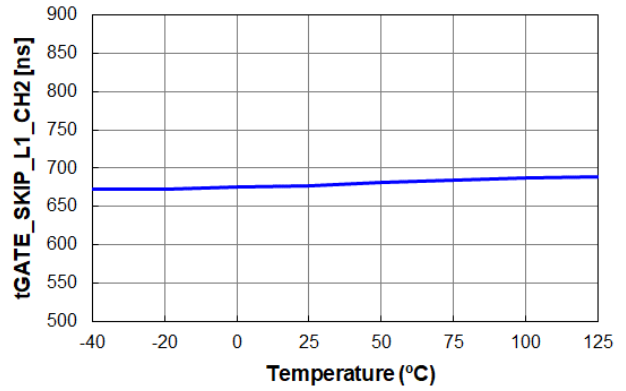
Figure 40. t_{\text{GATE-SKIP}_L1\_CH2} vs. Temperature
