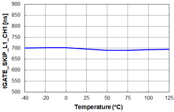
Figure 39. t_{\text{GATE-SKIP}_L1\_CH1} vs. Temperature
