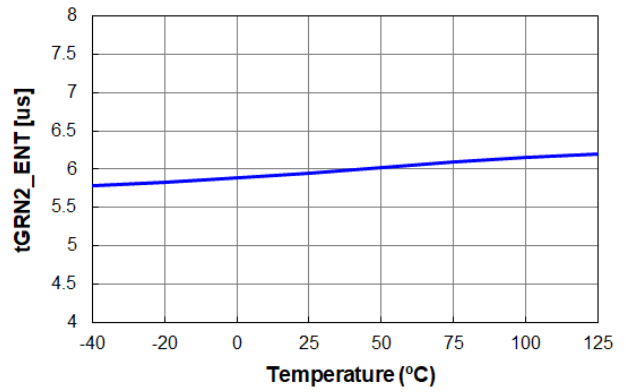
Figure 42. t_{\text{GRN2-ENT}} vs. Temperature
