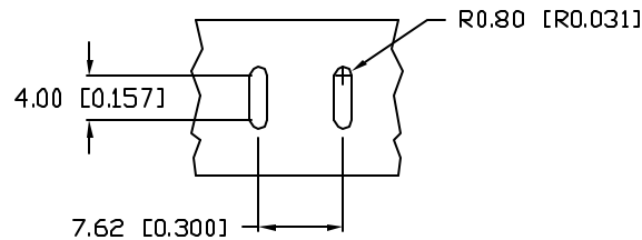
RECOMMENDED PCB CUT OUT
