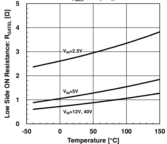
Low Side ON Resistance vs. Temperature (I_{GATE}=50mA(\text{Sink}))
