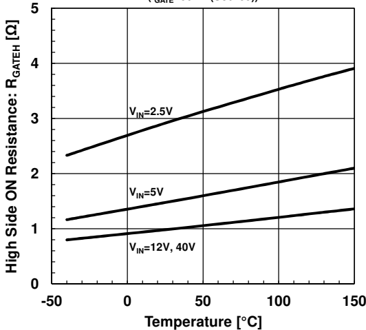
High Side ON Resistance vs. Temperature (I_{GATE}=50mA(\text{Source}))
