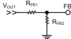
Figure 11: Connecting a Feedback Divider to Set the Output Voltage
