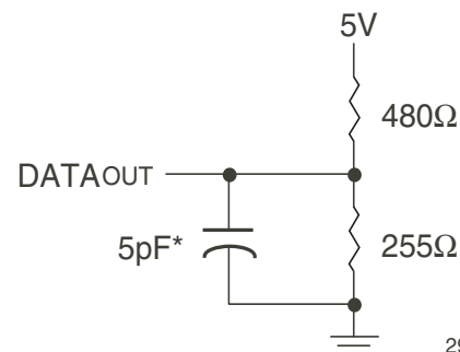
Figure 2. AC Test Load (for tOLZ, tOLZ, tCHZ, tOHZ, tOW, and tWHZ)
