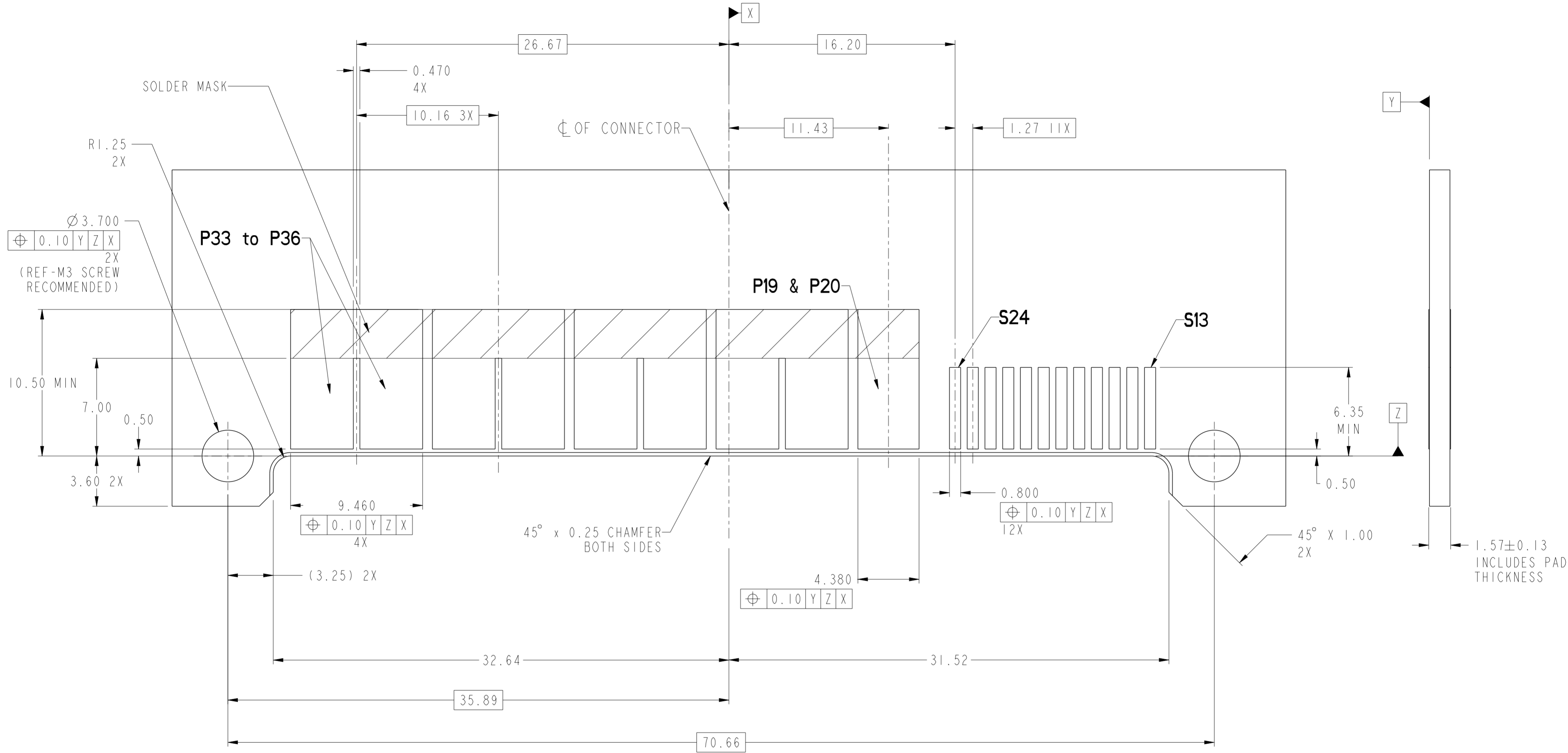
HOST BOARD LAYOUT AS VIEWED
